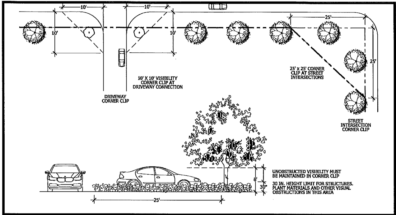
Figure 6-1 Visibility Triangle
